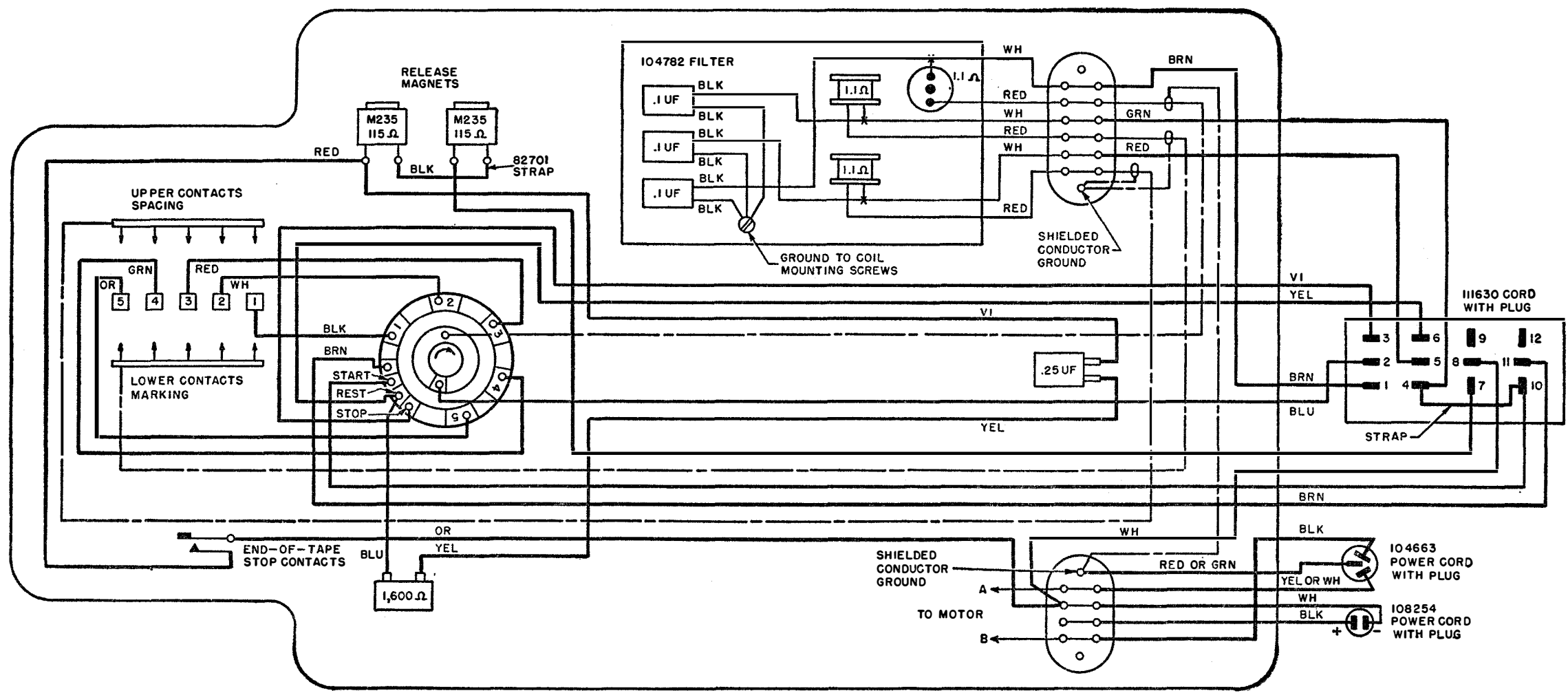
Figure 99. Transmitter Distributor TT-25/FG (receiving), wiring diagram.
