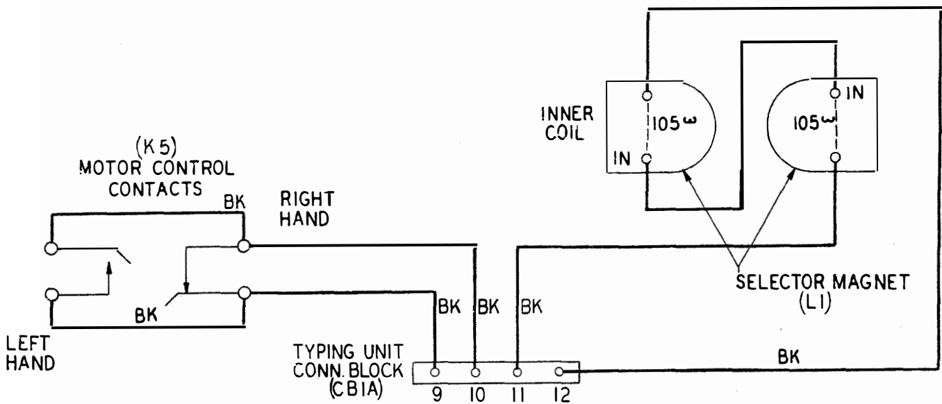
Figure 2 — 15B, 15D, 15F, 15H, 15K, 15M, 15N, and 15P Typing Units
