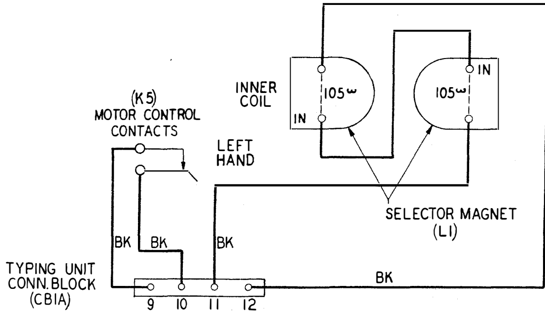
Figure 3 - 15J and 15L Typing Units
