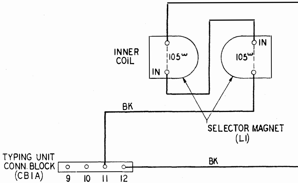
Figure 1 — 15A, 15C, 15E, 15G, 15R, 15S, and 15T Typing Units
