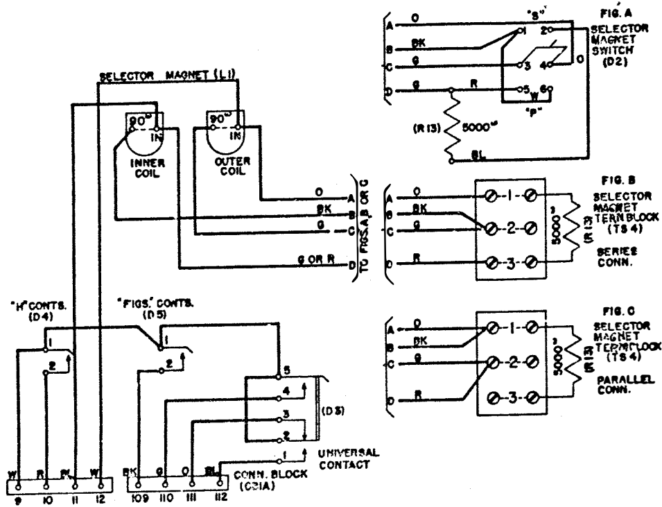
Figure 5 - 15AB and 15AD Typing Units
