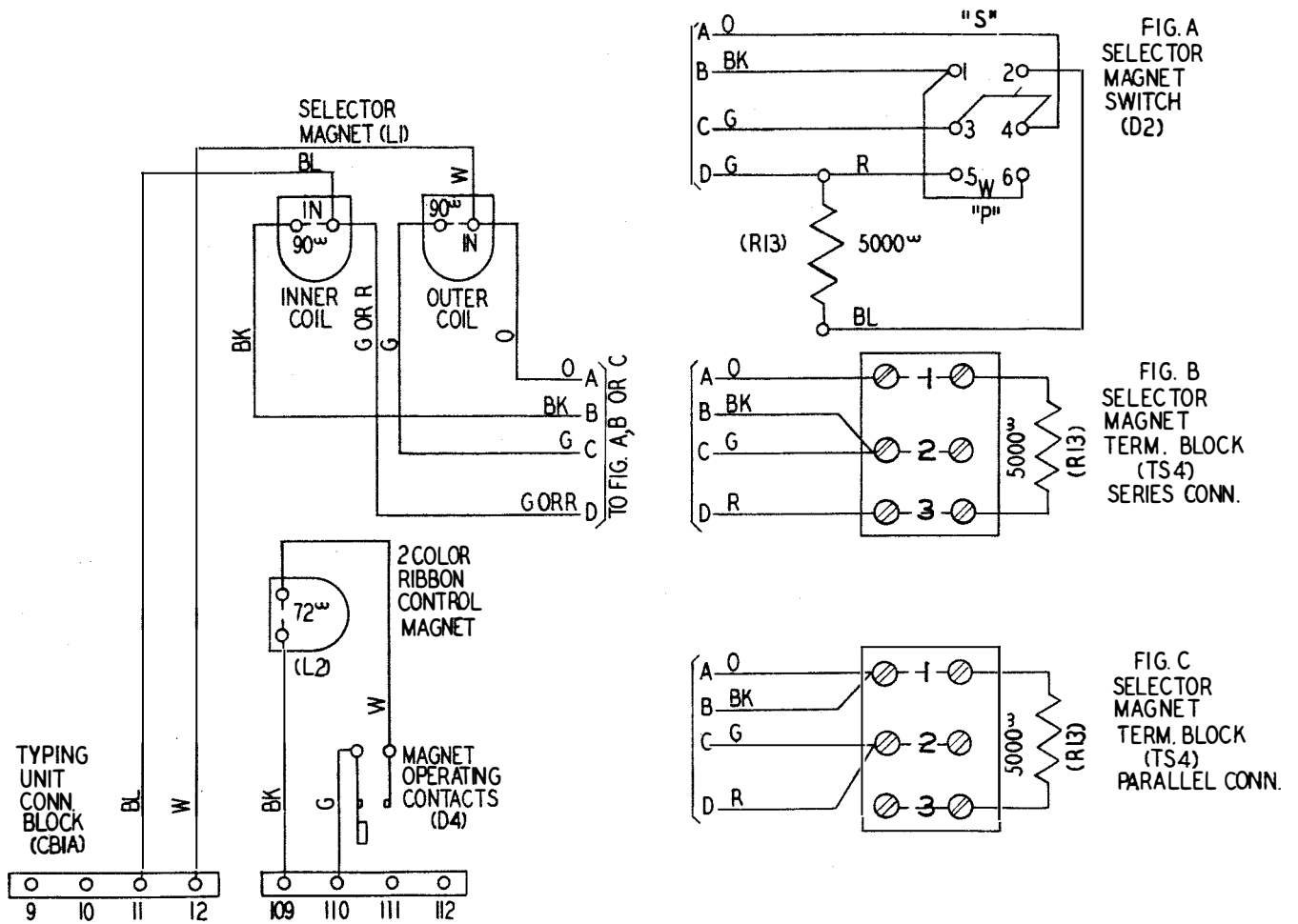
Figure 6 - 15AK Typing Unit
