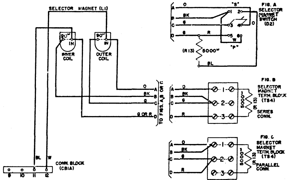
Figure 4 - 15U, 15W, 15Y, 15AA, 15AE, 15AF, 15AG, and 15AH Typing Units
