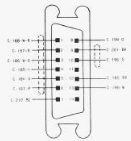
AD 161525 CONNECTOR PLUS
