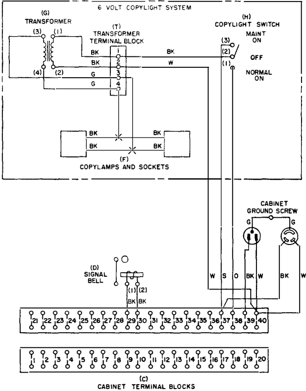
28LB Teletypewriter Cabinet
