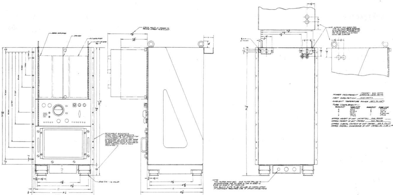
TRANSMITTING SET RADIO AN/URT-11(XN-1)
