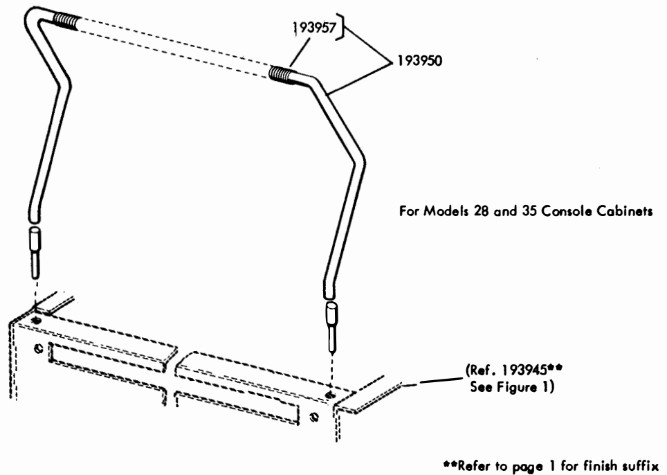
FIGURE 3. COPY DISPLAY RACK
