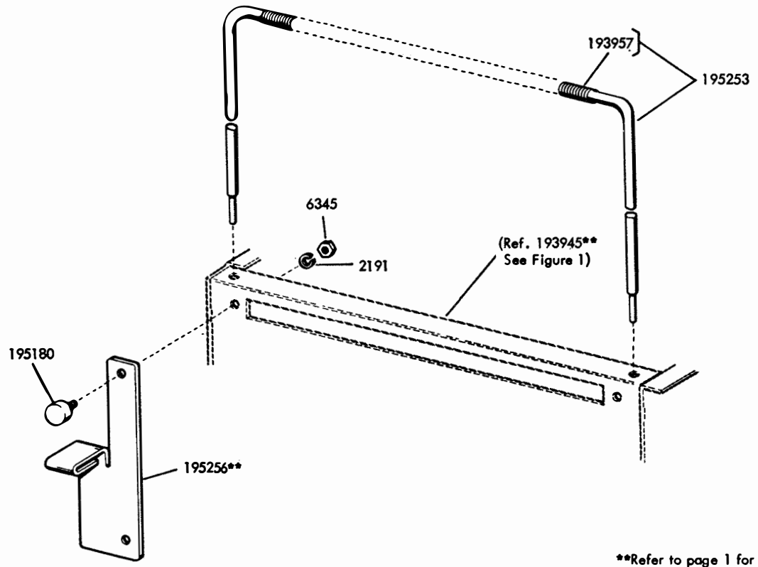
FIGURE 2. 195259** MODIFICATION KIT TO MOUNT PAPER WINDER AND PROVIDE COPY DISPLAY FOR MODELS 32 AND 33 PAGE PRINTERS
