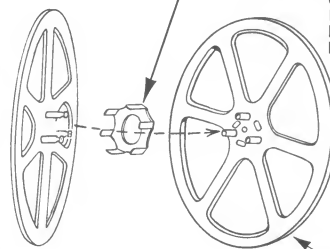
USE 4 1/2-INCH ADAPTER 146806 IF TAPE IS TO BE TRANSFERRED TO A REEL WITH A 4 1/2-INCH DIAMETER CORE
