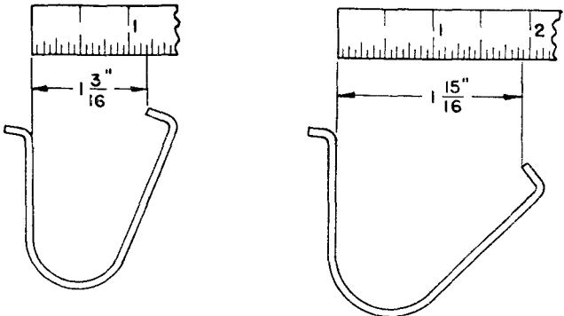
KEY LEVER SPRING
