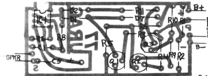
PARTS SIDE
