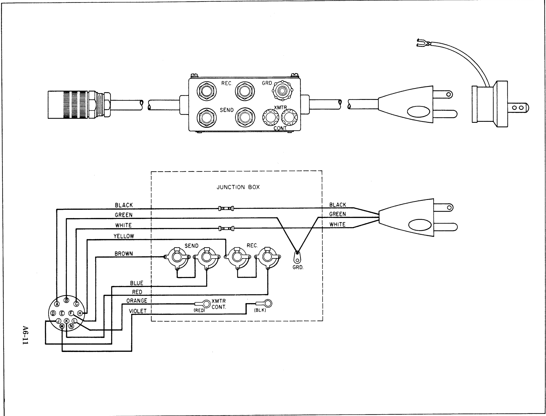
Figure A4-3. Bench Test Cable
