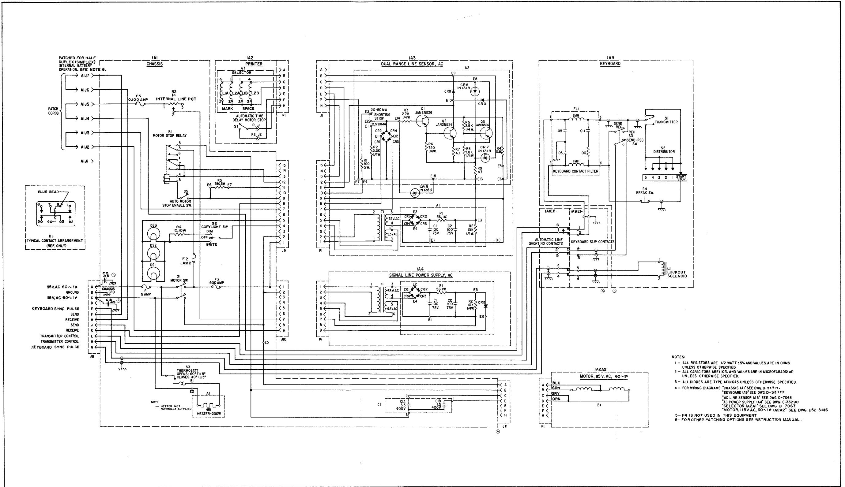
Figure A4-1. Schematic Diagram TT-299B/UG
