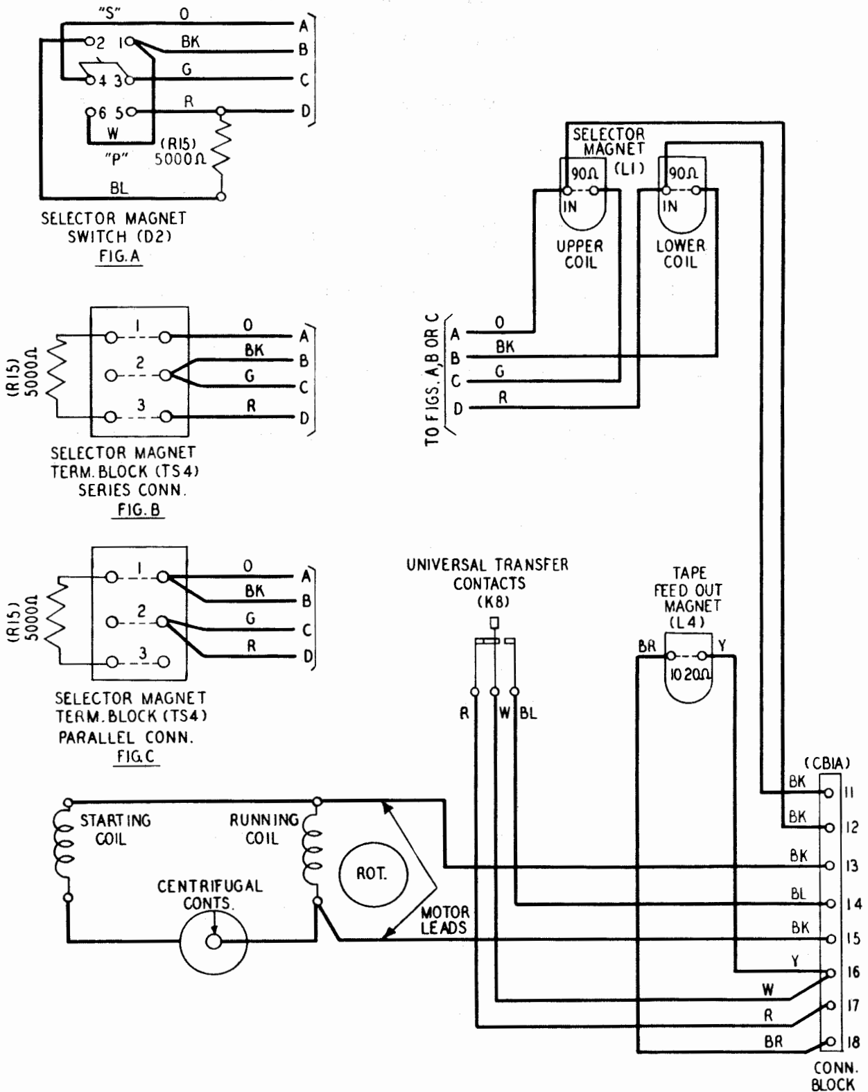
Figure 1 - 14AP, 14AP2, 14AR, 14AR1, and 14AT Typing Reperforator Units (Synchronous Motor)
