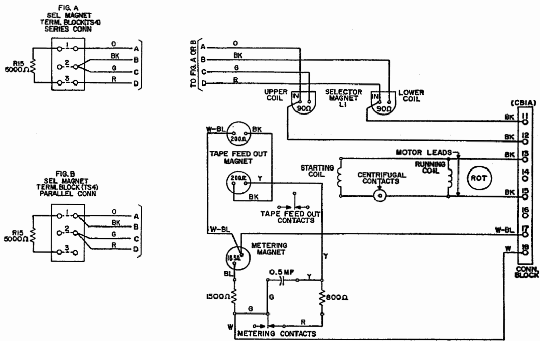
Figure 2 - 14AS Typing Reperforator Unit (Synchronous Motor)
