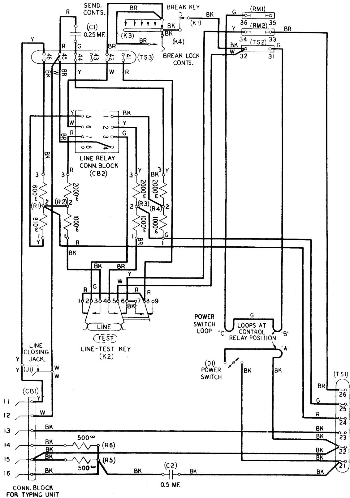
Figure 1 — 14B and 14T Teletypewriter Bases
