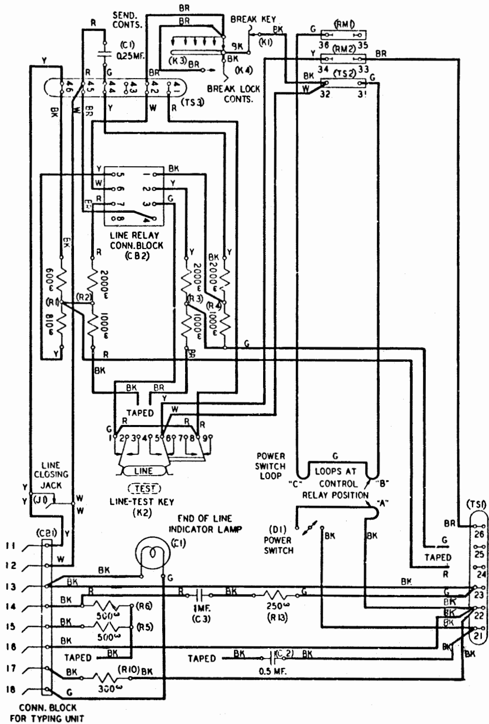
Figure 7 — 14N and 14P Teletypewriter Bases
