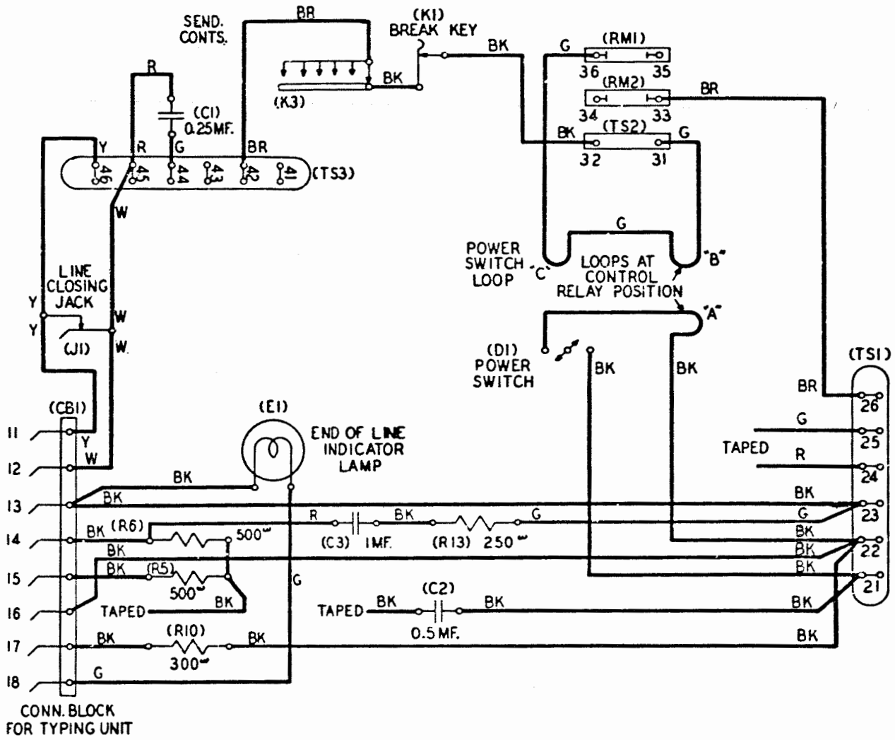
Figure 8 - 14R Teletypewriter Base
