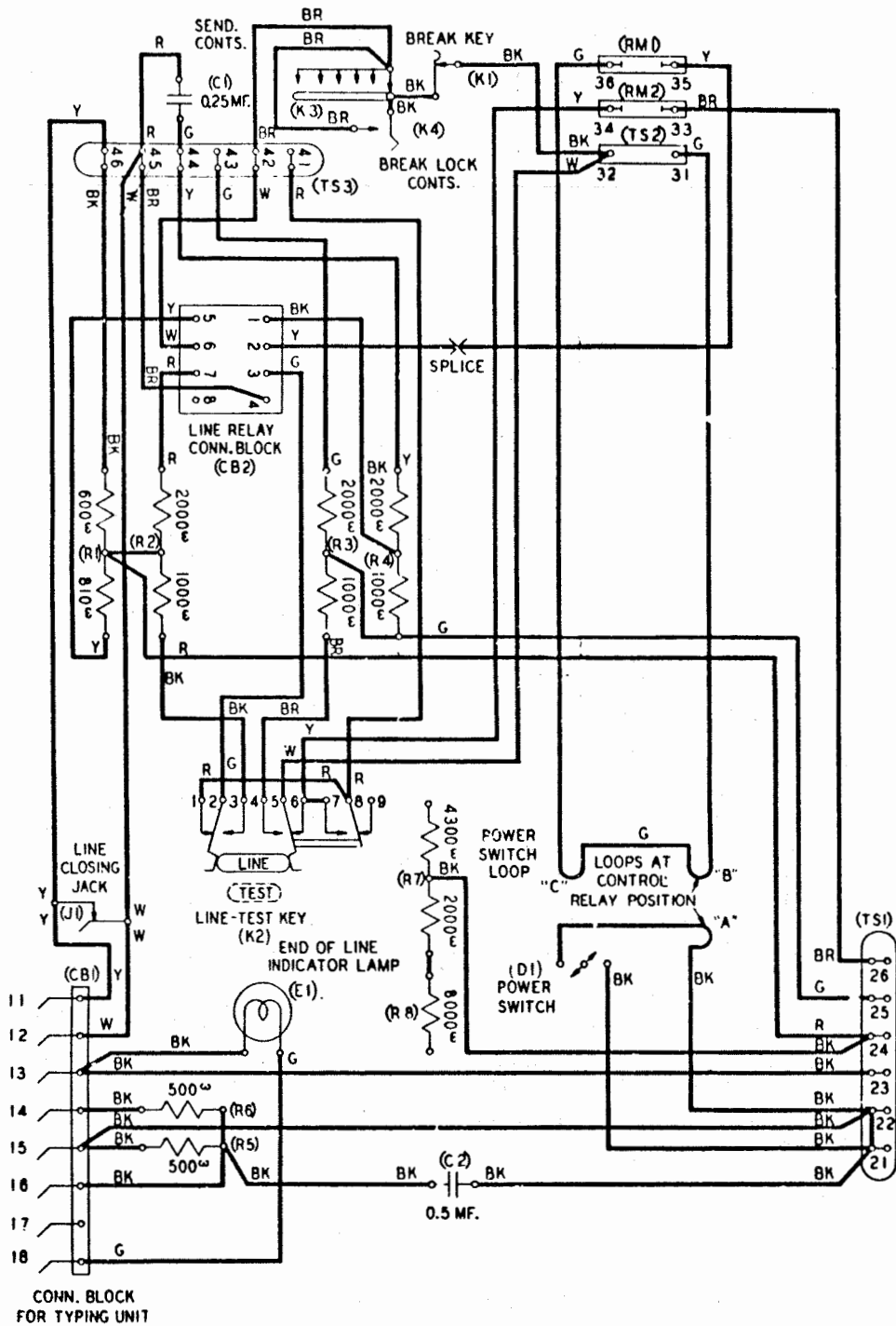
Figure 6 — 14M Teletypewriter Base
