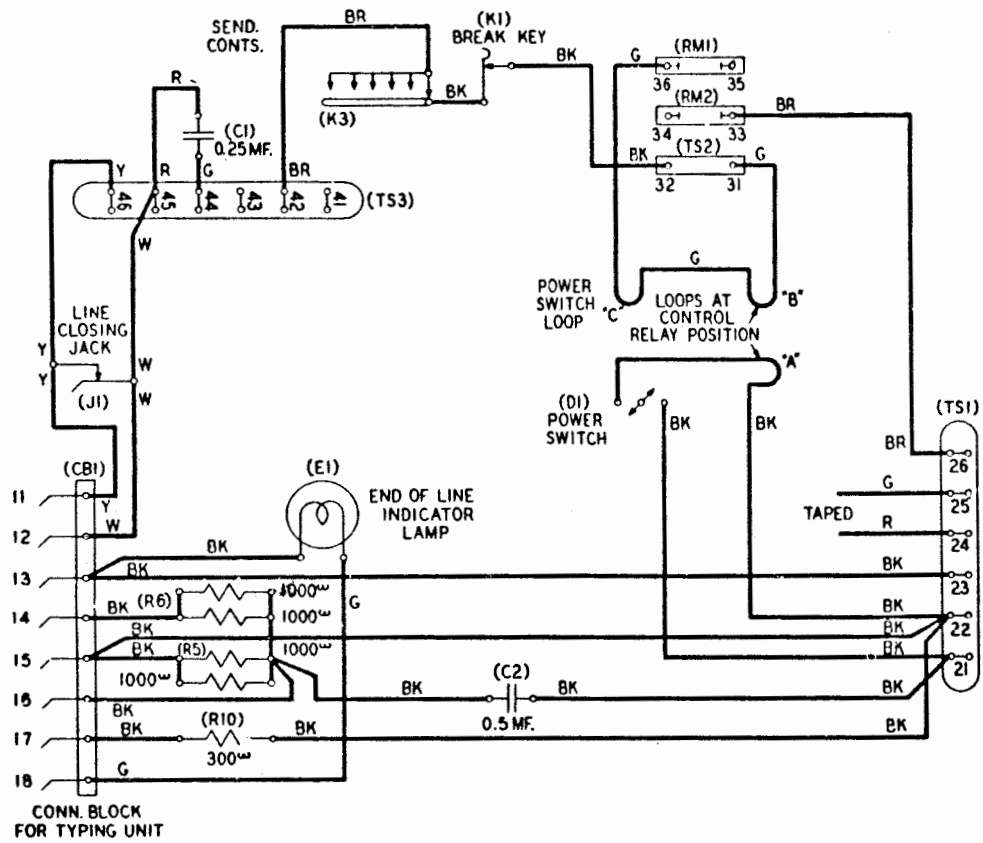
Figure 3 -- 14J Teletypewriter Base
