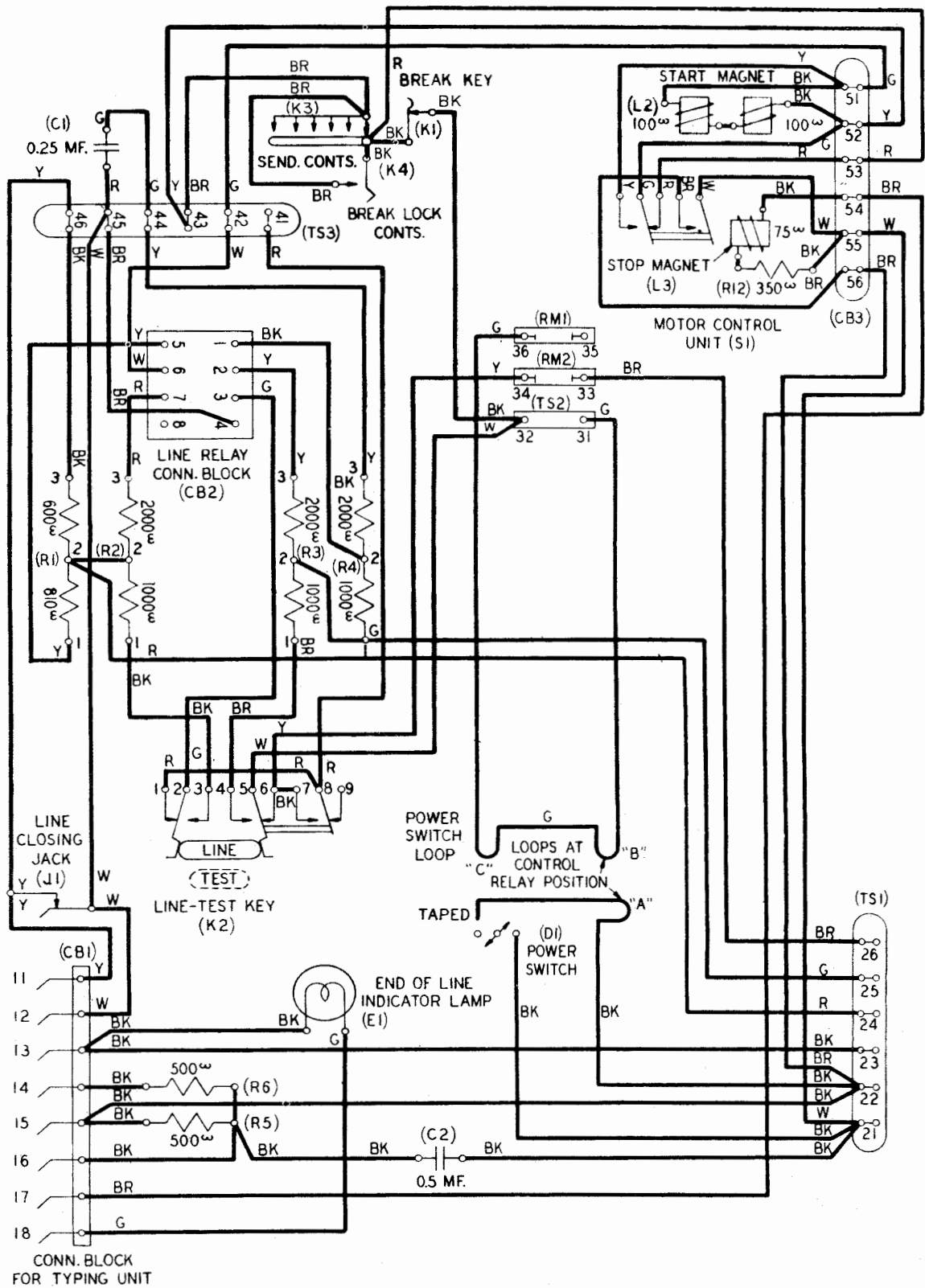
Figure 5 - 14L Teletypewriter Base
