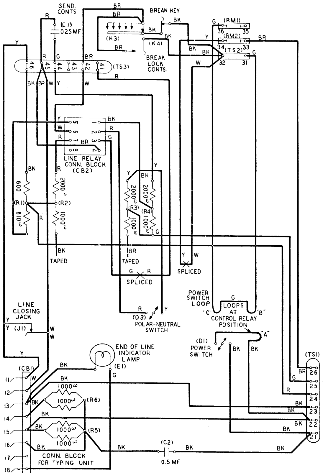
Figure 9 - 14U Teletypewriter Base
