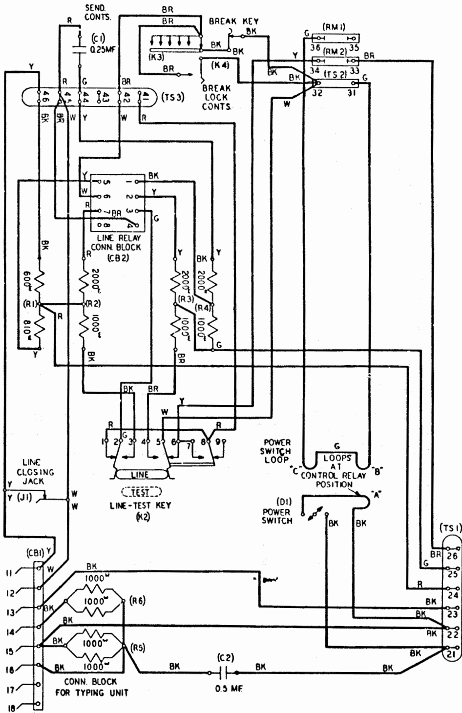
Figure 2 - 14H Teletypewriter Base
