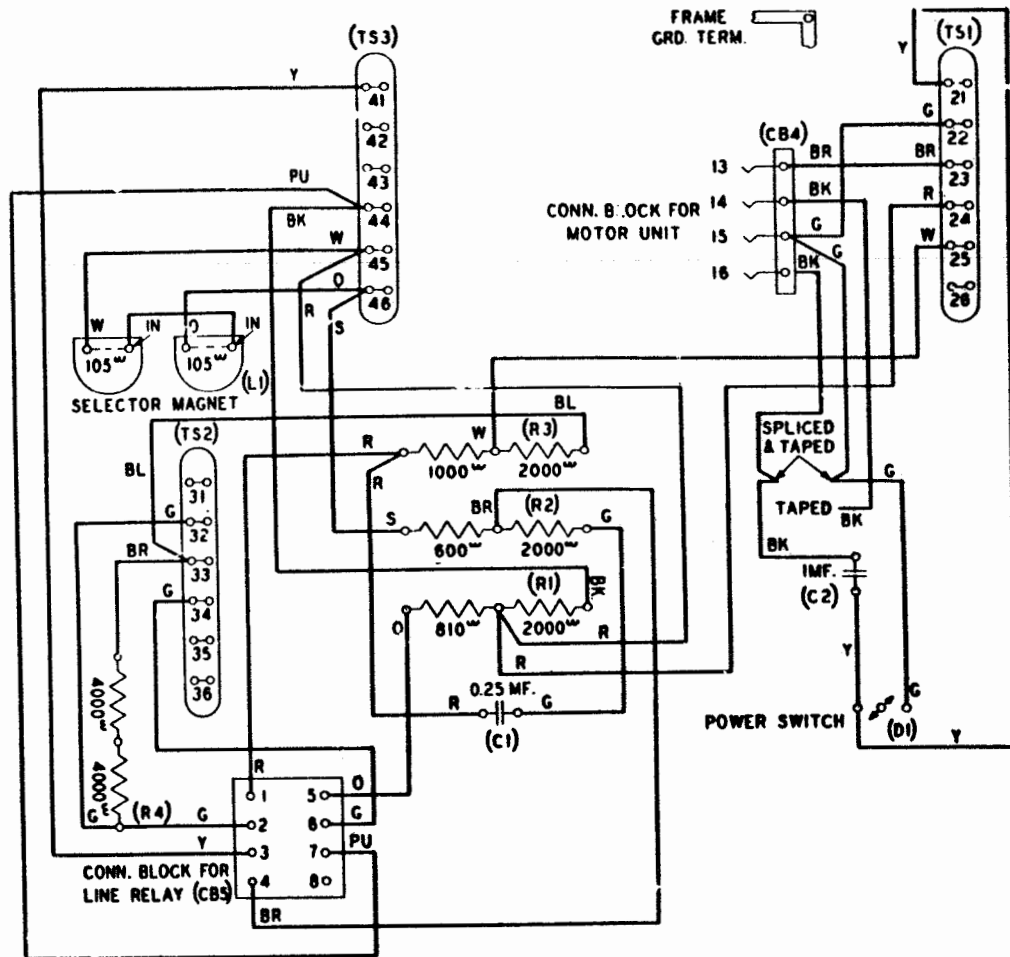
Figure 2 - 20 Reperforator Unit (14A Reperforator Unit - Later Design)
