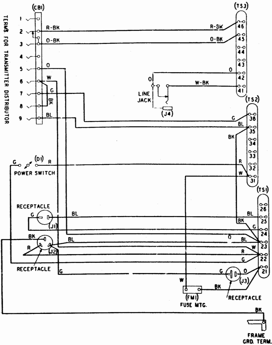
Figure 3 - 20 Reperforator Base (14A Reperforator Base Plate)
