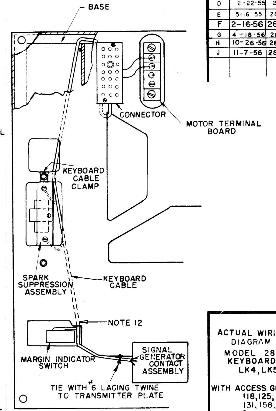
LK 5 BASIC CABLE ROUTING (TOP VIEW)
