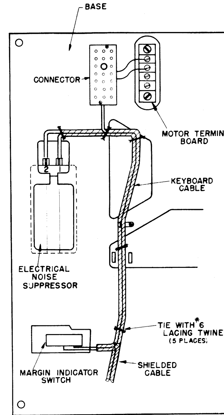
LK 4 BASIC CABLE ROUTING (TOP VIEW)
