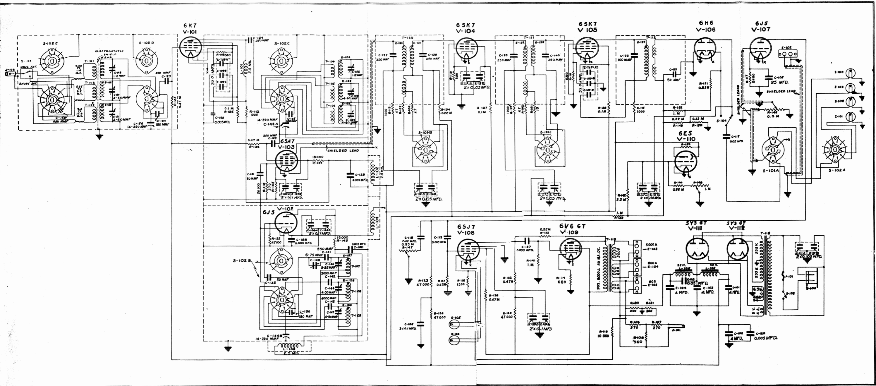
Schematic Diagram Type CZC-46225A Radio Receiver Model RB0-3
