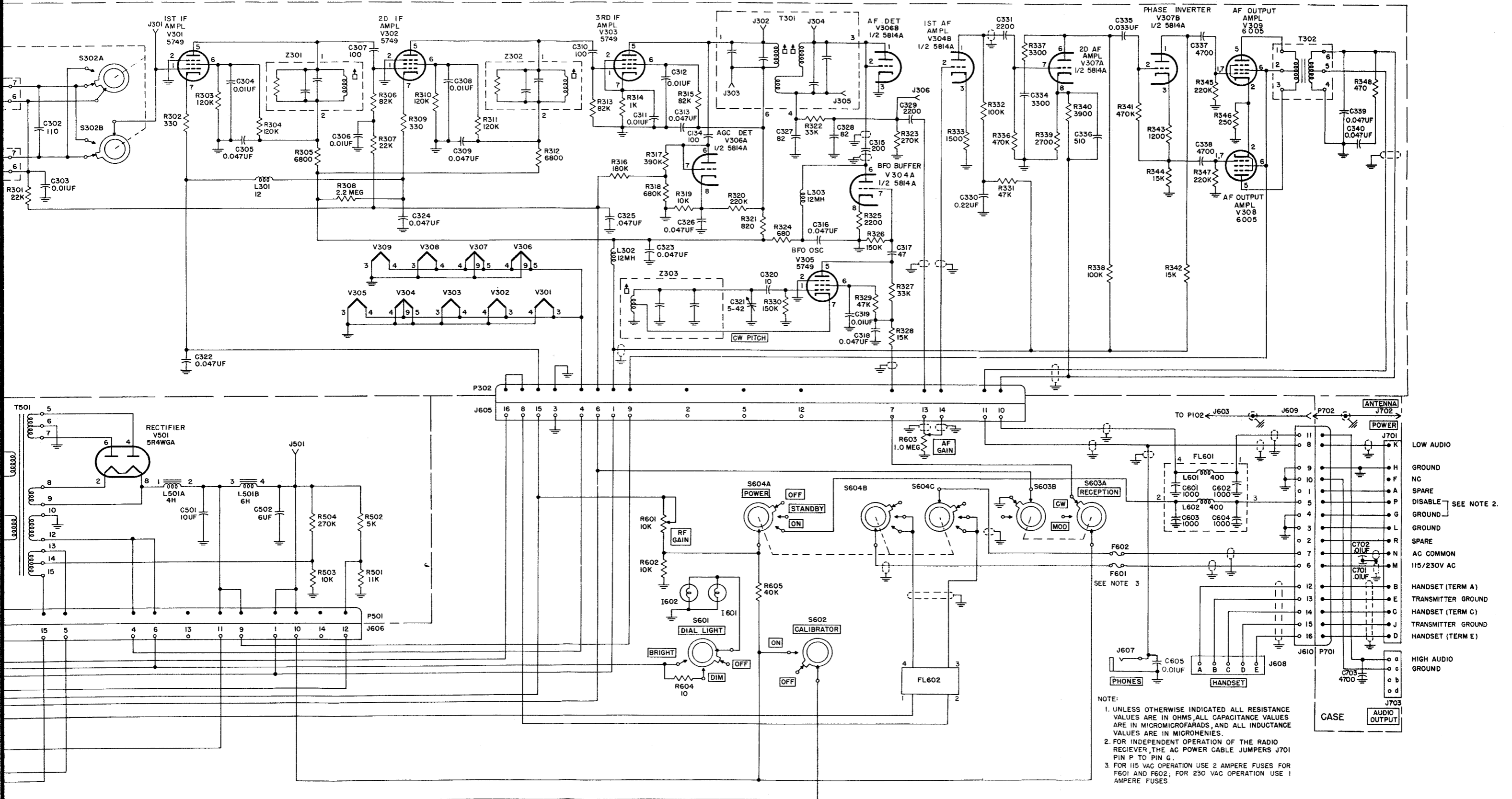
Figure 5-6. Radio Receiver R-627(XN-1)/URC-8, Schematic Diagram
